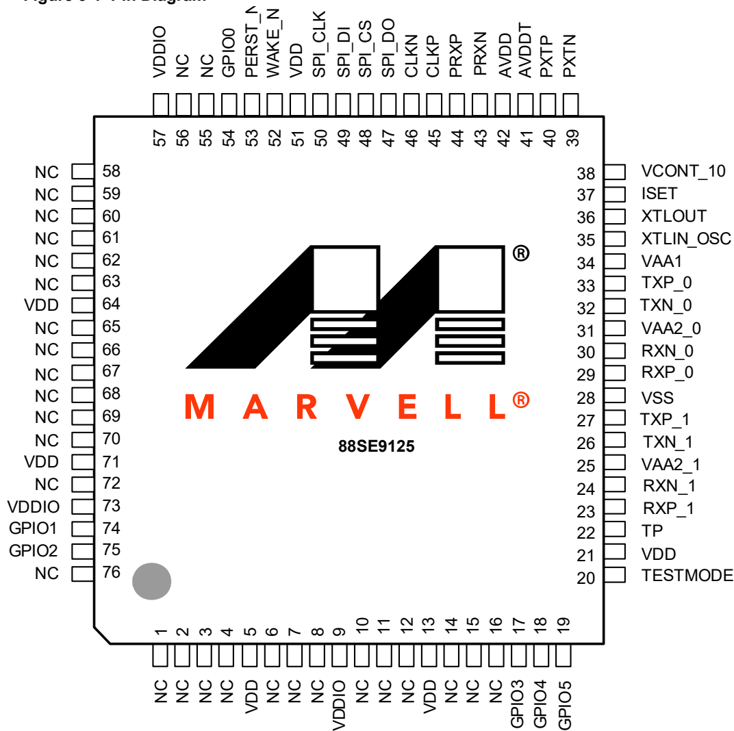
Figure 3-1 Pin Diagram
